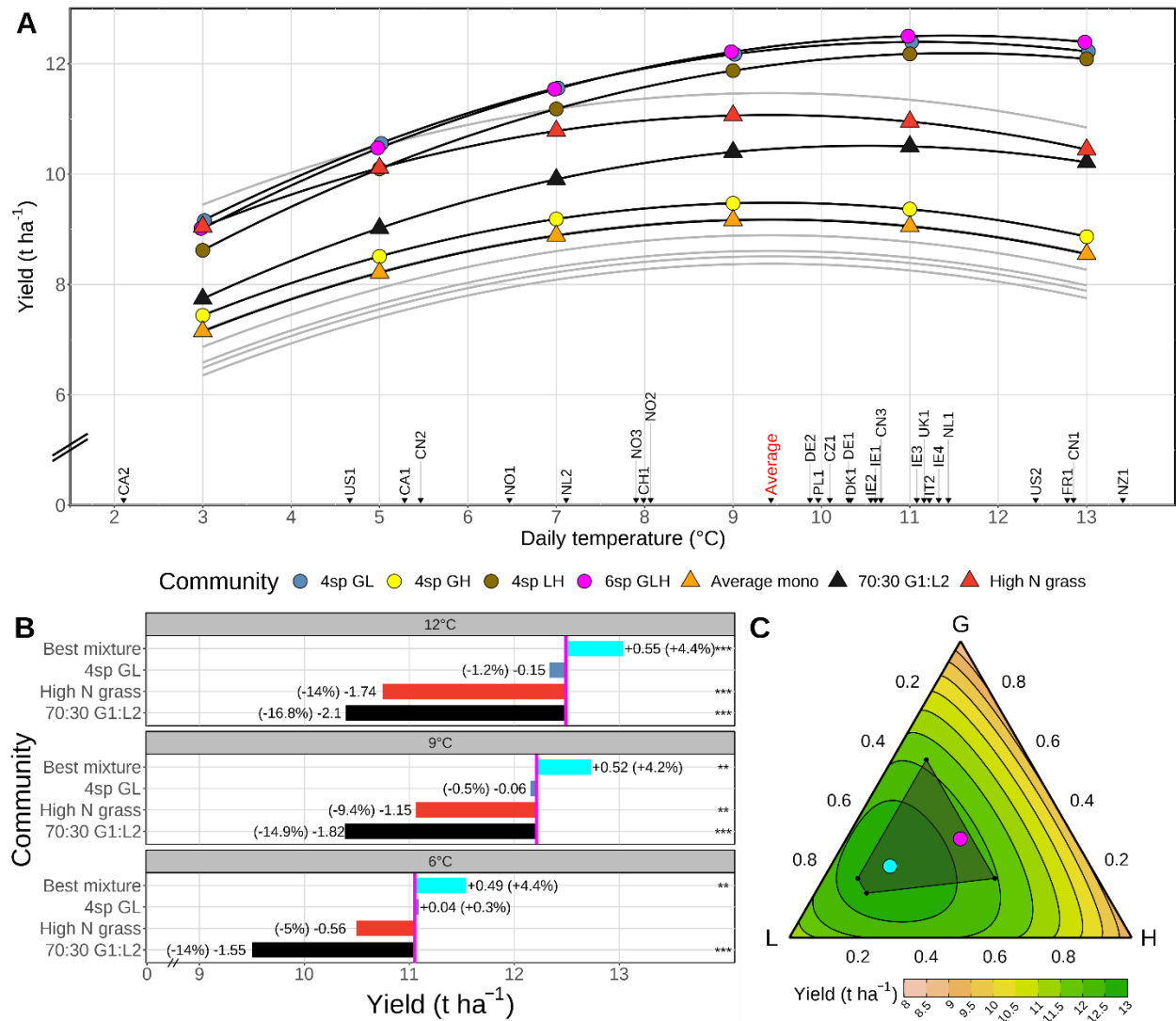
Fig. 4. As mean site temperatures increased, multispecies mixtures best maintained yield. (A) Predicted yields across the gradient of 3^{\circ}\text{C} to 13^{\circ}\text{C} average daily temperature for selected communities: the four-species equi-proportional mixtures of grass-legume, grass-herb and legume-herb (blue, yellow and brown circles, respectively), the six-species equi-proportional mixture of grass, legume and herb (magenta circle), the average of the six monocultures (orange triangle), the two-species 70:30 G1:L2 community (black triangle), and the high N grass monoculture (red triangle). Grey curves show the predicted yields of the six monoculture species (from highest- to lowest-yielding these are L1, H1, L2, G1, H2, G2). Circles on the top two curves are jittered. Site ID labels (Data S1) are included along the x-axis to indicate the average daily temperature at each site during the experimental period, the across-site average of daily temperatures is indicated as ‘Average’ (in red). (B) The predicted yield ( \text{t ha}^{-1} ) for the equi-proportional six-species mixture for three average daily temperatures 3^{\circ}\text{C} , 9^{\circ}\text{C} and 12^{\circ}\text{C} (vertical magenta line in each panel). For each temperature, differences are shown between the six-species equi-proportional mixture and each of four selected communities (as labeled on the y-axis): 70:30 G1:L2 community (black), high N grass (red), four-species equi-proportional grass-legume mixture (blue), and the optimal ‘best’ mixture (cyan). Significant differences are
