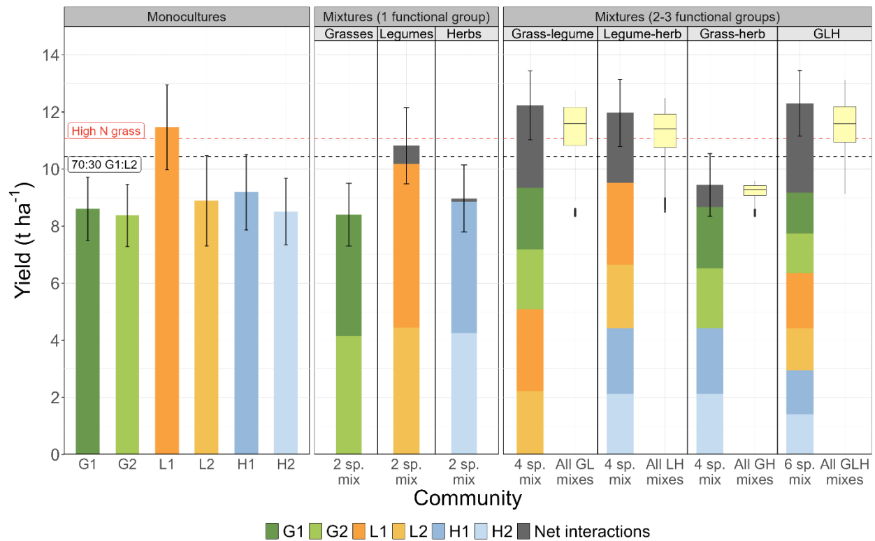
Fig. 2. Yields of monocultures and multispecies mixtures with varying functional group richness. Predicted yield per growing season ( \text{t ha}^{-1} ) for selected communities across sites (predicted from the model estimates in Table S2, n = 1,382 ). For each bar, yield predictions are broken down by the components of the model prediction (model species' identity effect estimates, each scaled by the respective sown proportion, plus scaled net interactions for mixtures; G1 = grass 1, G2 = grass 2, L1 = legume 1, L2 = legume 2, H1 = herb 1 and H2 = herb 2). The error bars show 95% confidence intervals for each prediction. The monoculture bars show predicted yield for the six monoculture communities. The 'Mixtures (1 functional group)' bars show predictions for the equi-proportional two-species mixtures where the two species are from the same functional group. For the G1:G2 equi-proportional mixture, the interaction term is negative and therefore not shown (effect = -0.09 \text{ t ha}^{-1} , \text{SE} = 0.17 ); the height of the bar represents the contribution of G1 and G2 to the yield, minus the negative interaction effect. The 'Mixtures (2–3 functional groups)' bars show predicted yields for the four-species equi-proportional GL, LH and GH mixtures, and the predicted yield of the six-species equi-proportional GLH mixture. The boxplots show the estimated distributions of predicted responses for all possible GL mixtures, LH mixtures, GH mixtures, and GLH mixtures. The dashed red line is the predicted yield of the high N grass monoculture. The dashed black line is the predicted yield of a 70:30 G1:L2 two-species community, where G1 was L. perenne and L2 was T. repens at the majority of sites.
