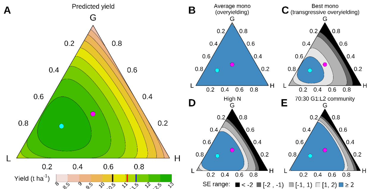
Fig. 3. Higher yields from increased plant diversity. (A) Ternary diagram illustrating predicted yield (t ha -1 ) across all sites as the sown proportions of the three functional groups vary, and with the two species within each functional group sown in equal proportions to each other. Note that the vertices of the ternary are two-species communities of grasses (G), legumes (L), or herbs (H), not monocultures of individual species. The highest predicted yield is marked by a cyan circle (with sown functional group proportions: G:L:H = 24:59:17 and corresponding sown species proportions = 0.12: 0.12: 0.295: 0.295: 0.085: 0.085). In the yield legend, values are marked for the predicted responses of the 70:30 G1:L2 community (black), the high N grass monoculture (red), and the highest yielding monoculture (blue). The predicted yield for the equi-proportional six-species mixture is shown by a magenta circle. The remaining panels show the difference (measured in standard errors) of the predicted yield in A from: (B) the weighted average monoculture (for the component species at each point in the ternary; overyielding), (C) the highest yielding monoculture (i.e., L1, which was T. pratense at most sites; transgressive overyielding), (D) the high N grass monoculture, and (E) the 70:30 G1:L2 two-species community, where G1 was L. perenne and L2 was T. repens at most sites. For example, a point on panel D within the highest contour level (colored blue) represents a mixture whose predicted yield is more than two standard errors greater than the predicted yield of the high N grass monoculture. The six-species equi-proportional mixture and the optimal mixture are marked in B to E for comparison to panel A.
